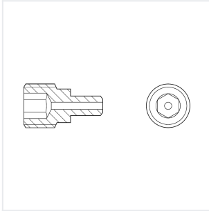
Hohlschraube M10x1x25-45H
